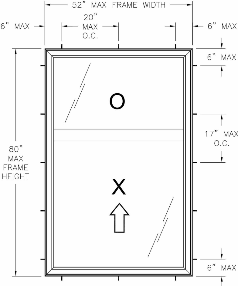
CAMBRIDGE REVERSE ORIEL SINGLE HUNG EXTERIOR VIEW FRAME INSTALLATION
