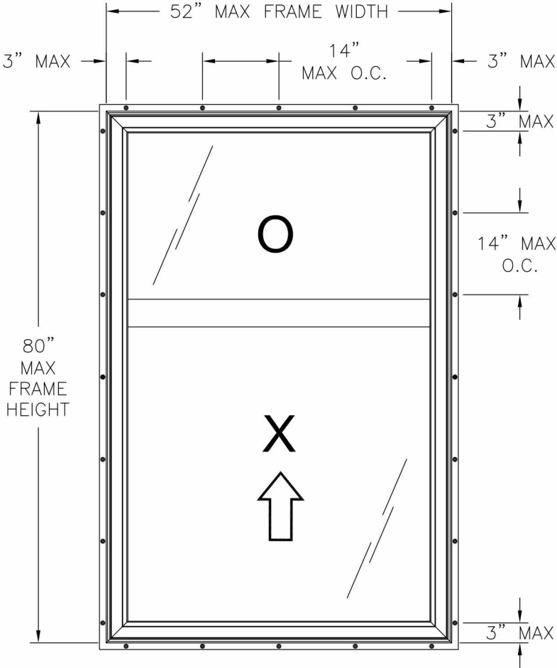
S-SERIES REVERSE ORIEL SINGLE HUNG EXTERIOR VIEW FIN INSTALLATION
